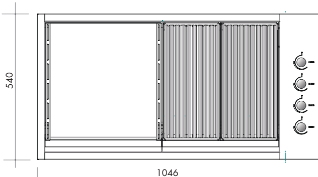
TOP VIEW ABBQM
