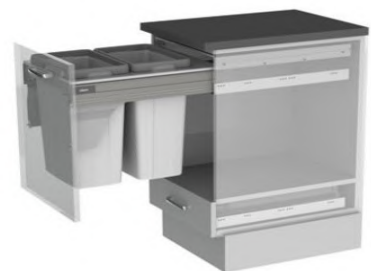
BINUB60035S – BIN FRAME SET 2 X 35LTR TO SUIT 600MM CABINET WIDTH 570H X 562-568W X 515D
