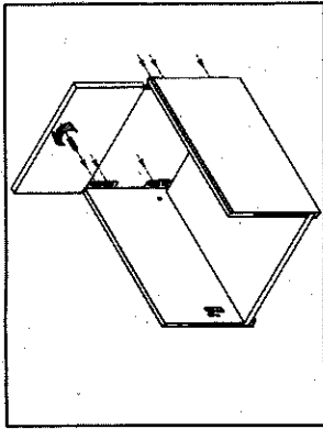
Back assembly
