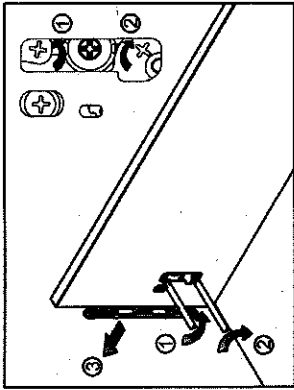
Front bracket release
