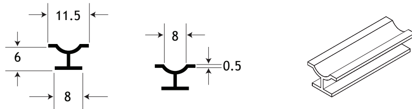
Sliding Door Ultra Lower Track (7H x 12W)
