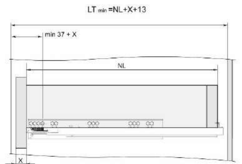
Built-in drawer
