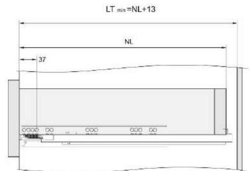
Standard drawer
