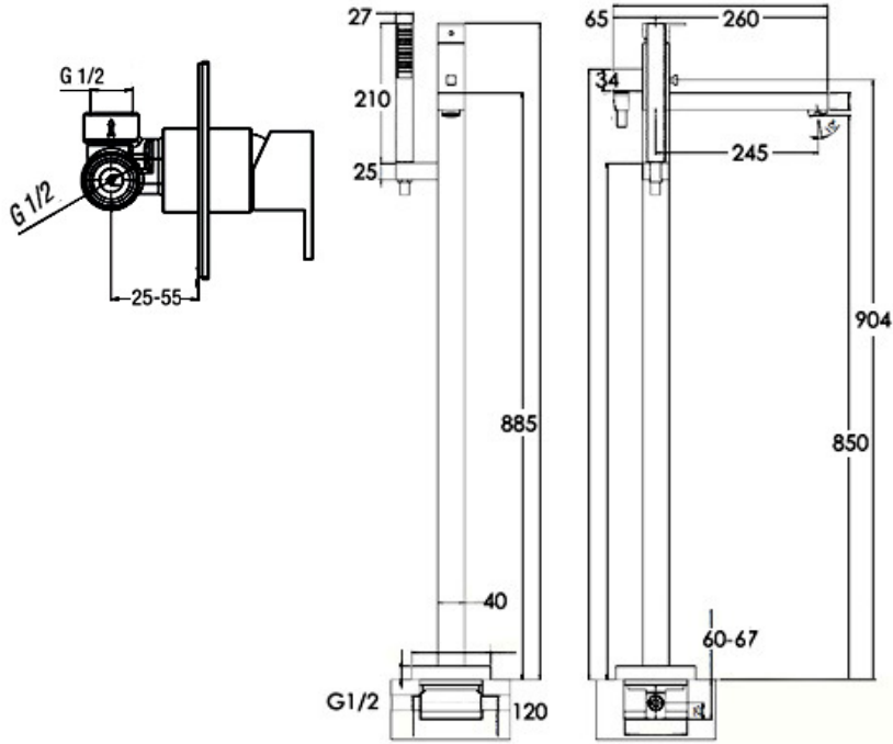
7300/C Freestanding Bath Spout Chrome
