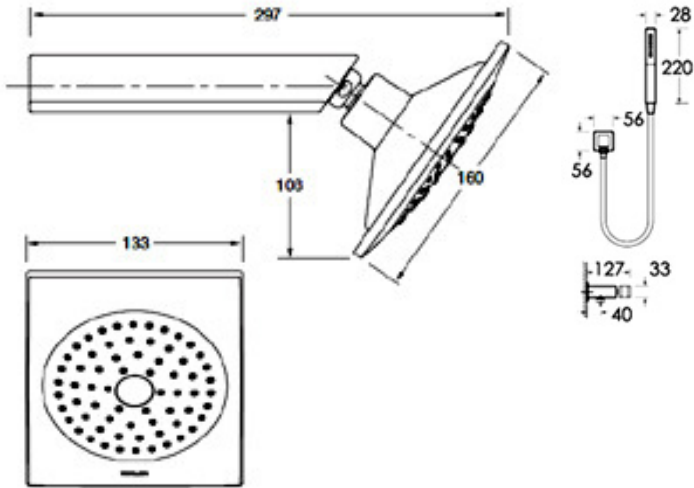
14787A-CP Overhead Shower Chrome
