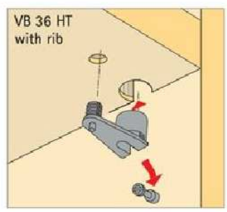
Fit shelf in position from above. Mounting aid when hanging shelves.
