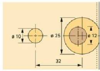
Fit shelf in position from above. Mounting aid when hanging shelves.
