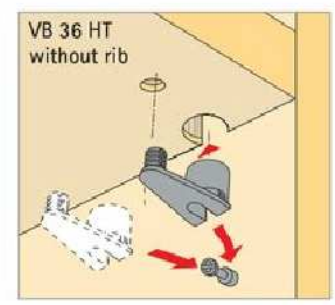
Fit shelf from above or the front
