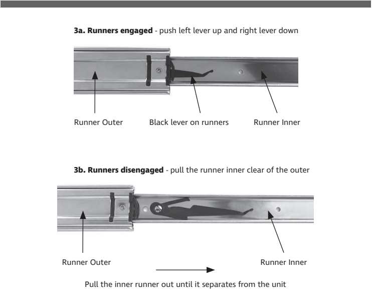
FIG 3a / 3b - Removing Runners
