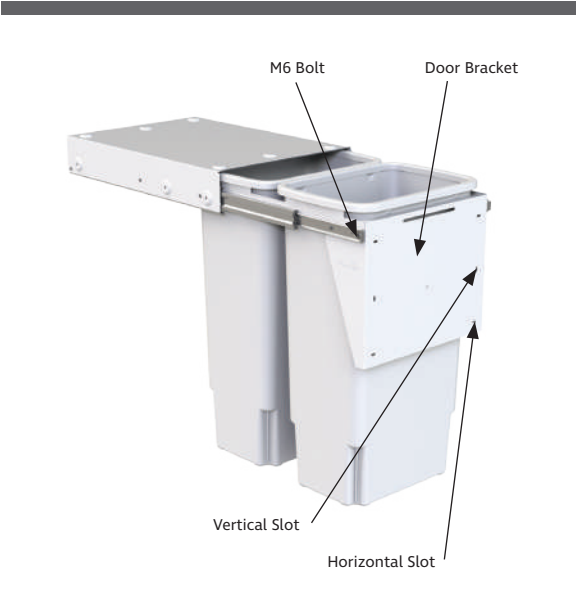
FIG 2 - Bin Parts for Door Pull Models
